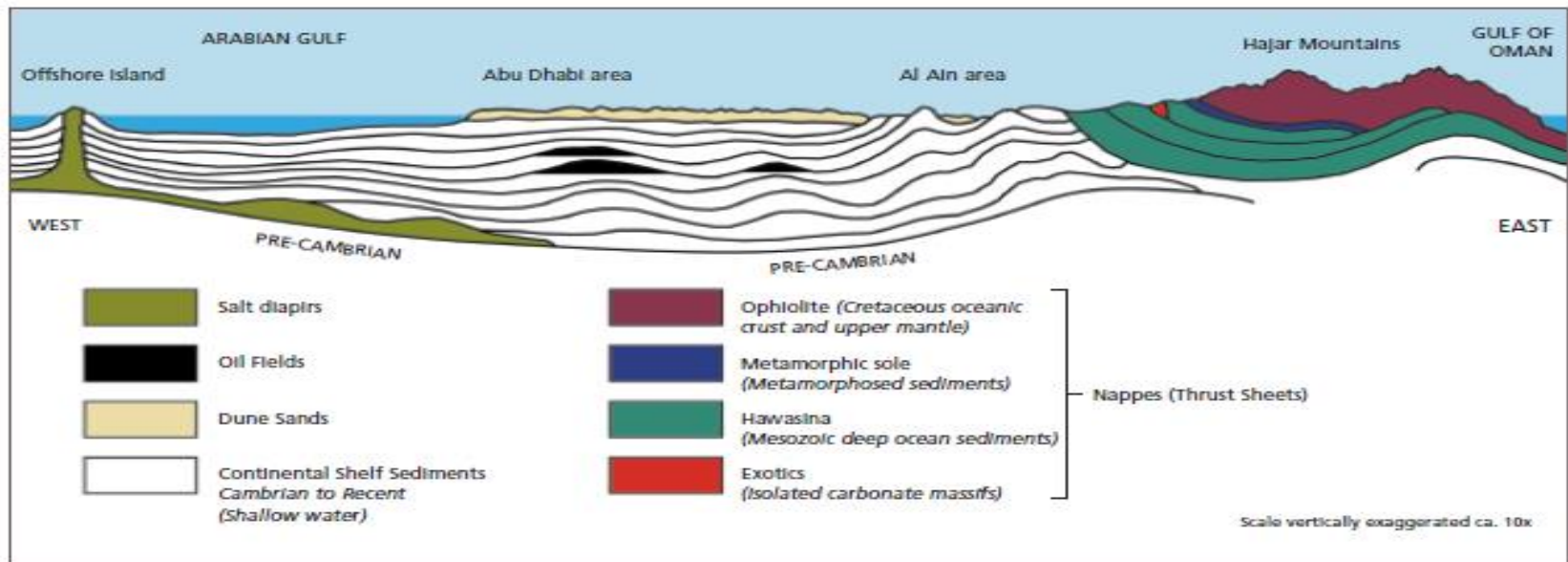
FIGURE 4: Geological cross-section of the UAE.
